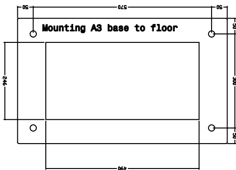
Standard base height 200 and 450mm
