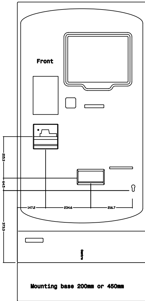
Mounting positions for A3 to Machine Base
