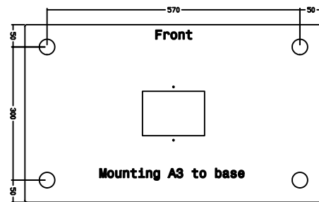
Standard base height 200 and 450mm
